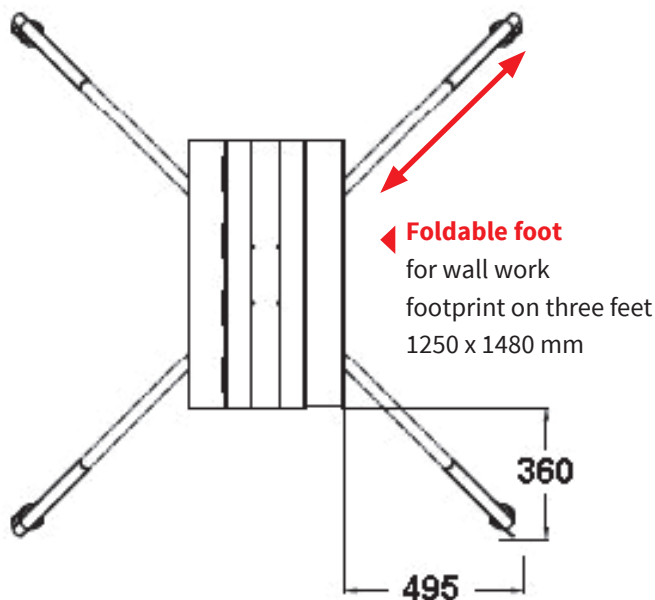
Manual use With crank provided
